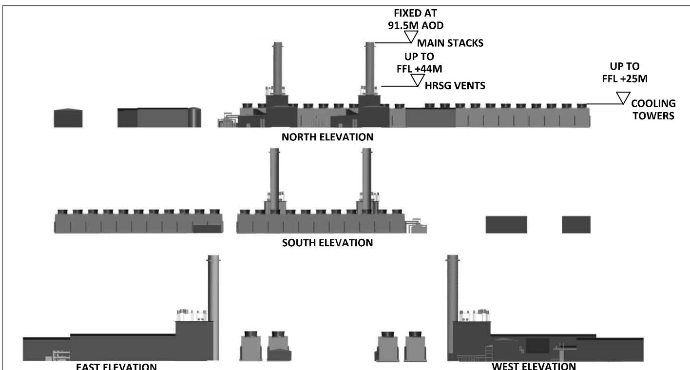
SHEET 3 OF 3 - ELEVATION VIEW
